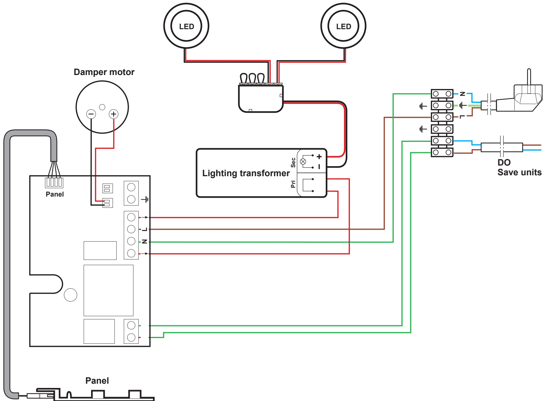
Wiring diagram 392-10
